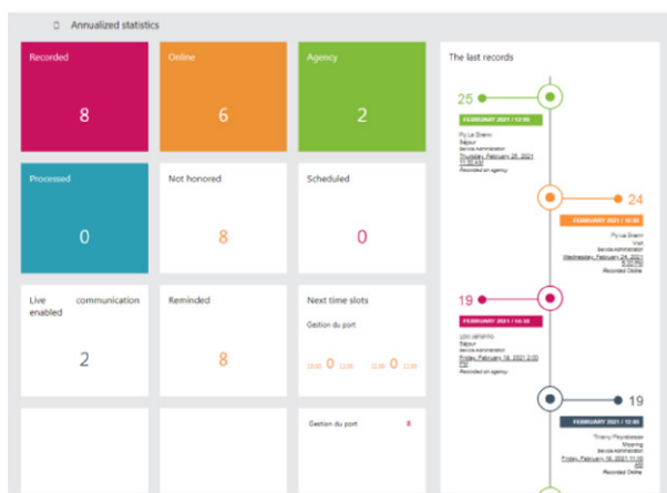
Figure 3. Statistics
