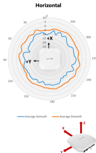
Azimuth plane (top view) – 6.50GHz
